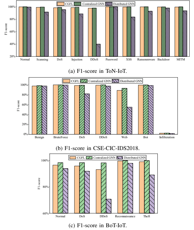
Fig. 4. F1-score of CGFL, Centralized GNN, Distributed GNN.
