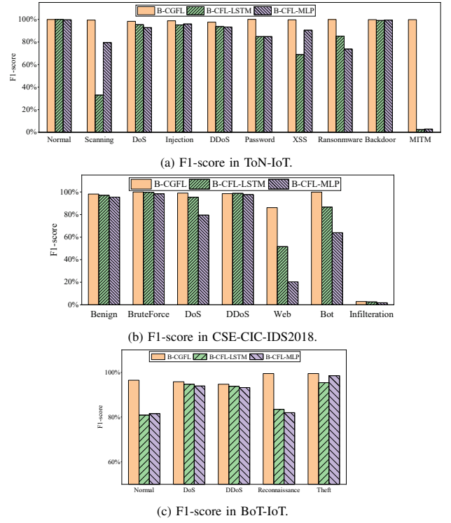
Fig. 6. F1-score of B-CGFL, B-CFL-LSTM, and B-CFL-MLP.
