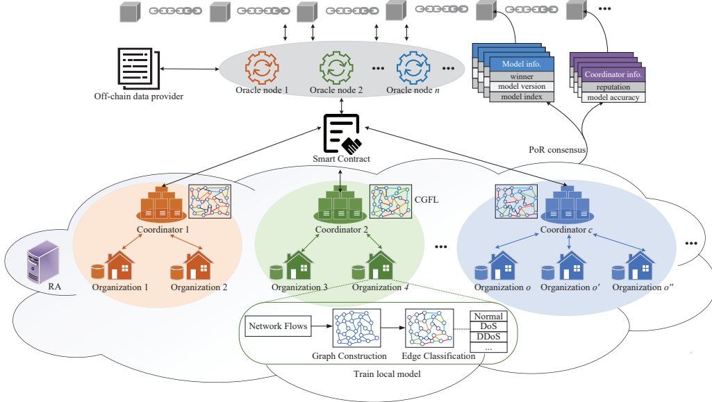
Fig. 1. Blockchain-enabled collaborative intrusion detection framework.
