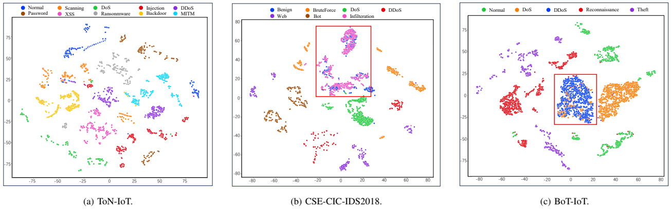
Fig. 7. Visualization analysis of network flow classification with B-CGFL.
