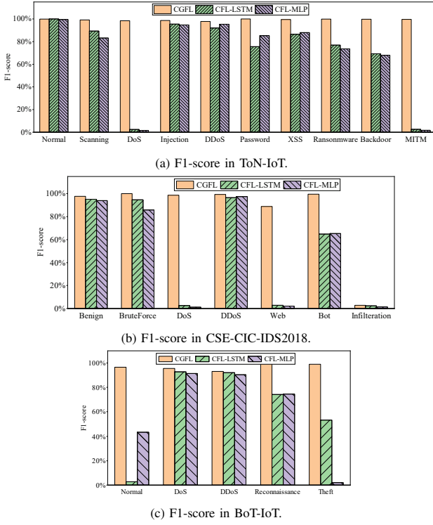
Fig. 5. F1-score of CGFL, CFL-LSTM, and CFL-MLP.
